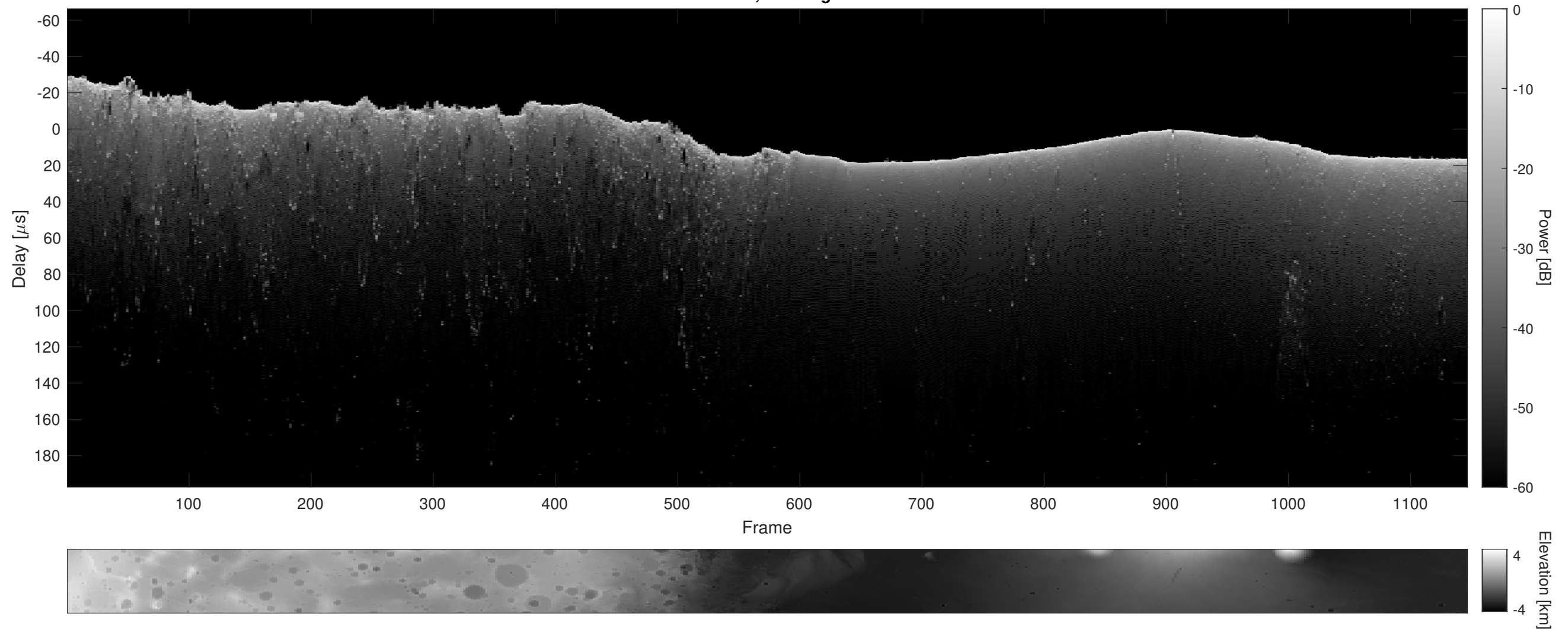
Orbit 8249, Cluttergram
