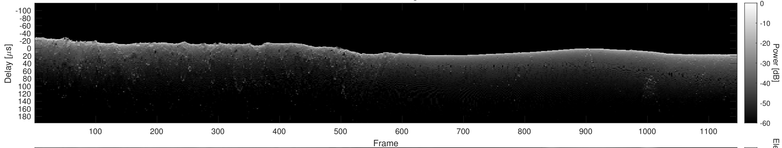
Orbit 8249, Cluttergram
