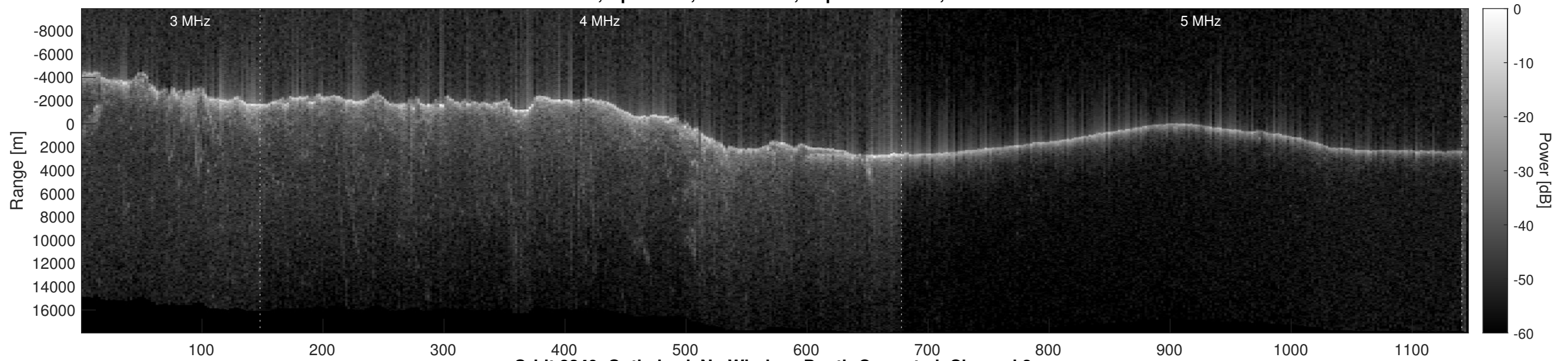
Orbit 8249, Optimized, No Window, Depth-Corrected, Channel 2
