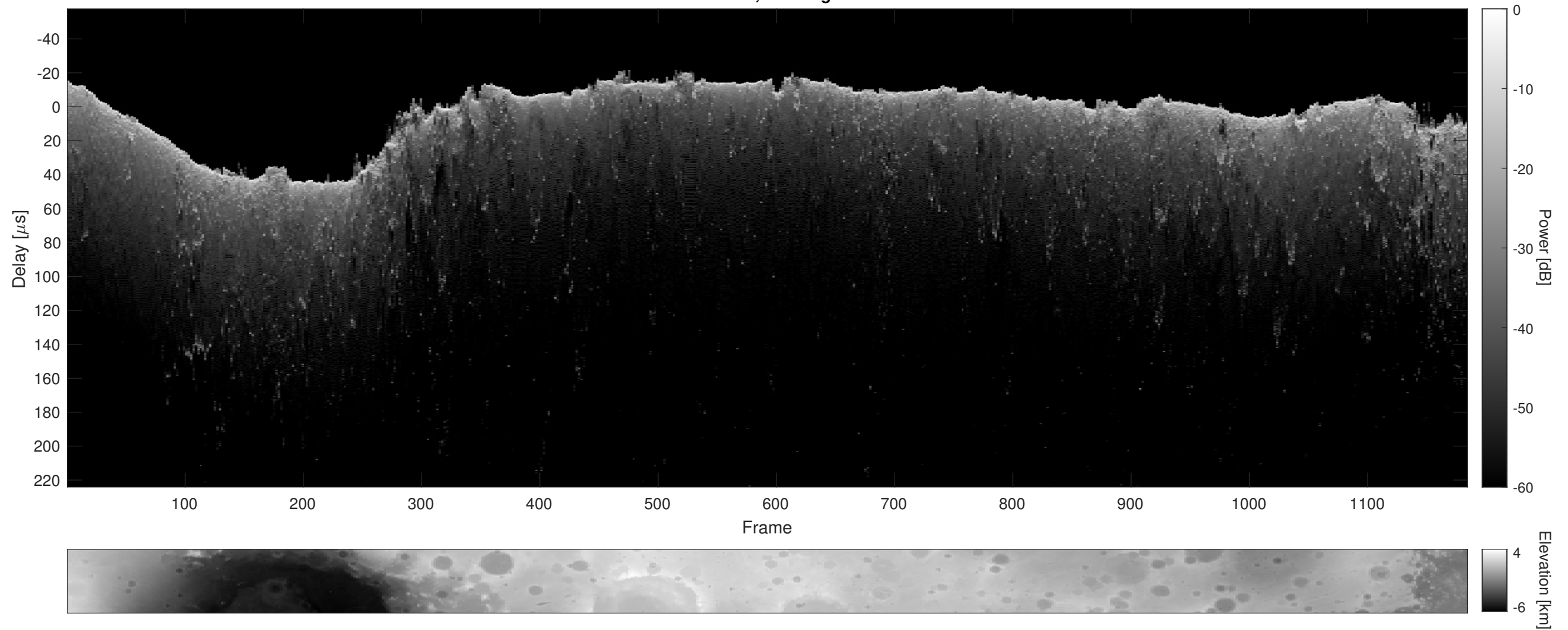
Orbit 8250, Cluttergram
