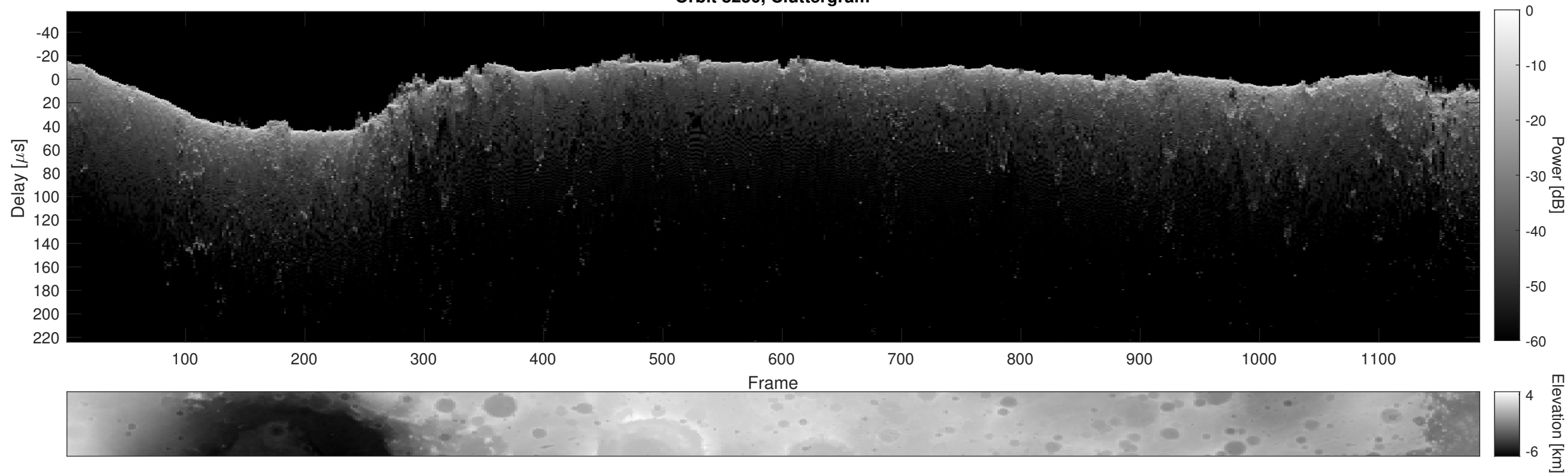
Orbit 8250, Cluttergram
