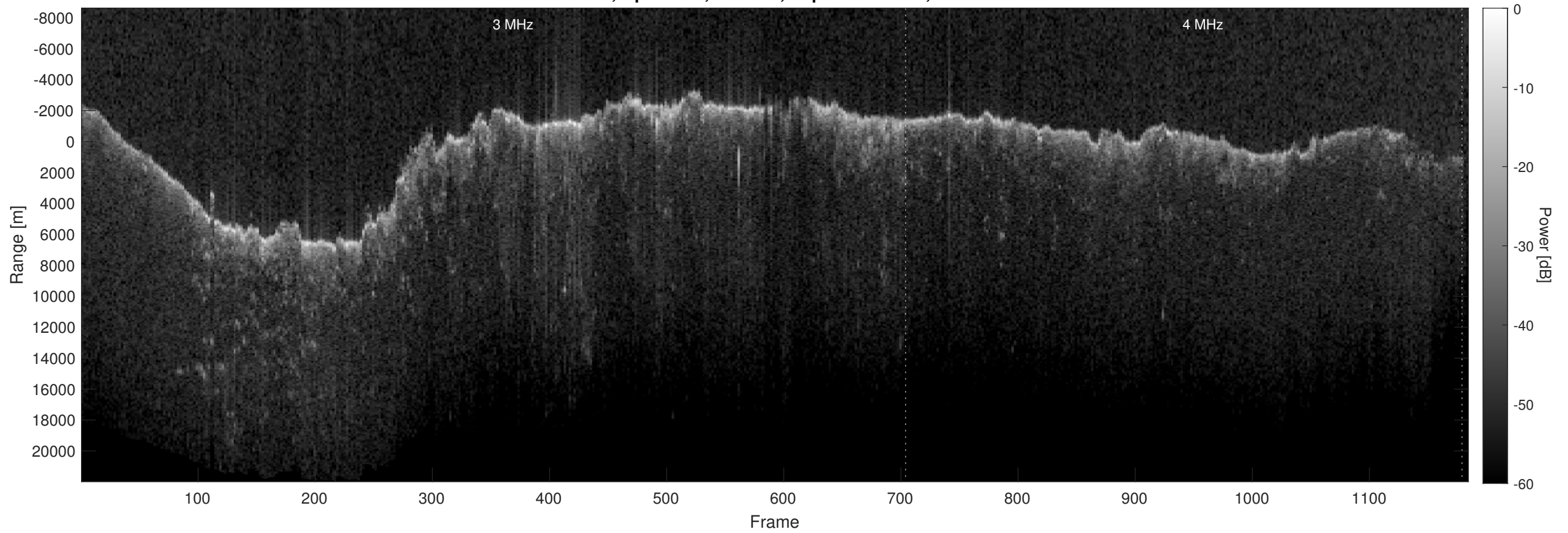
Orbit 8250, Optimized, Window, Depth-Corrected, Channel 2
