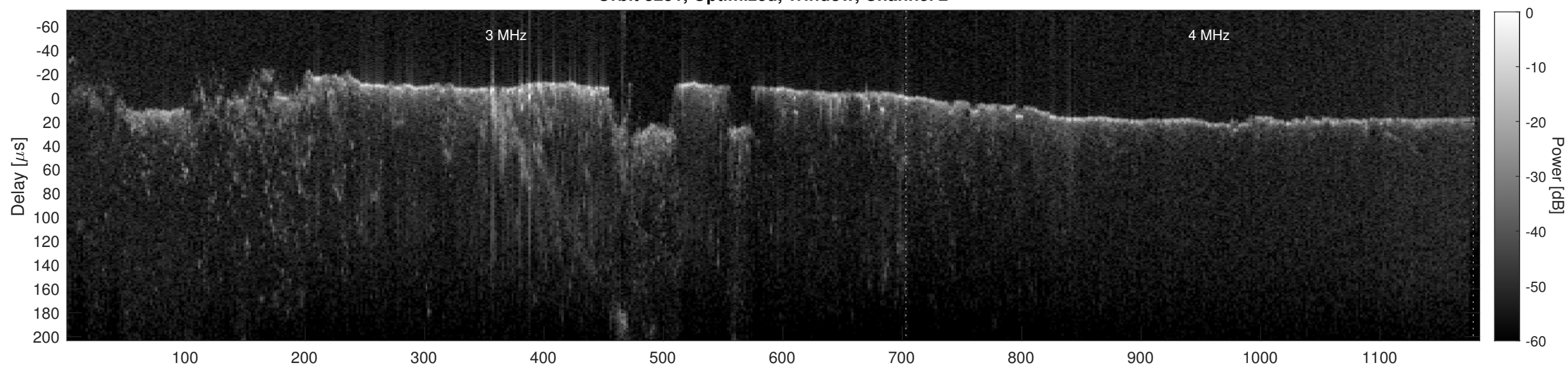
Orbit 8251, Cluttergram
