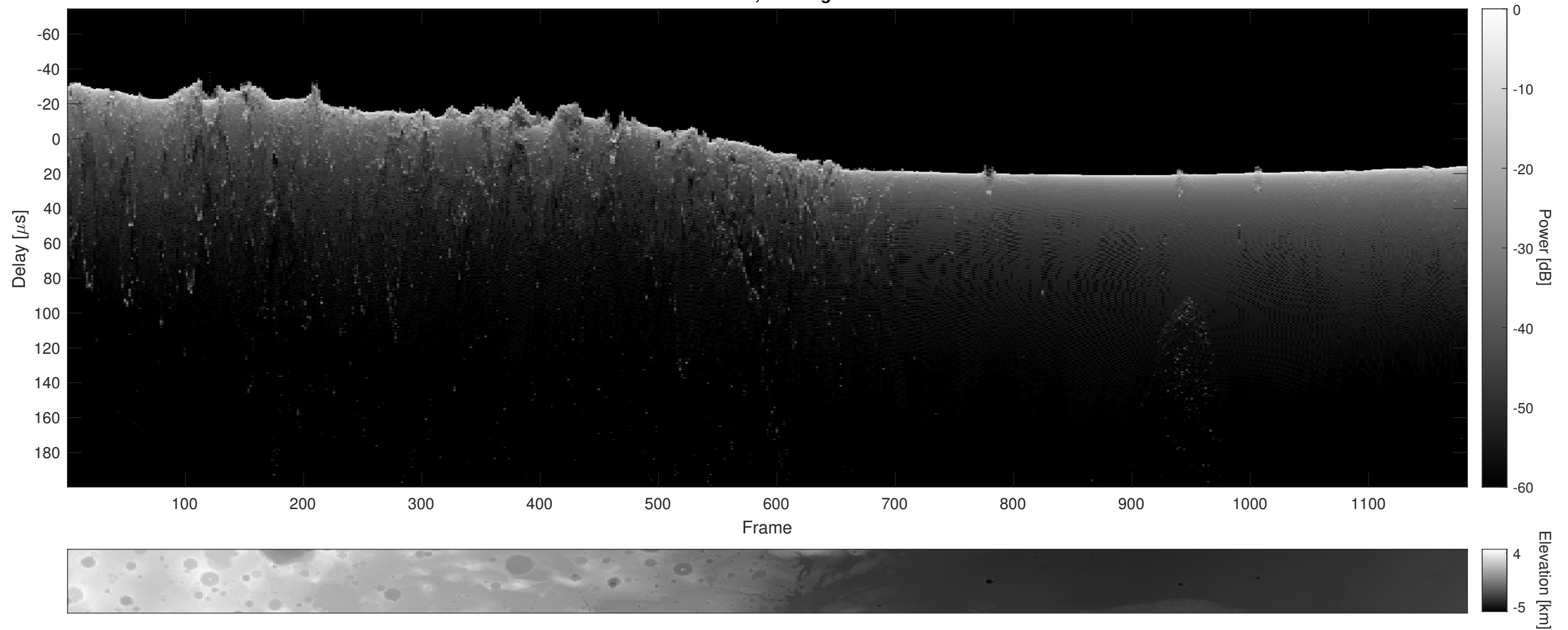
Orbit 8252, Cluttergram
