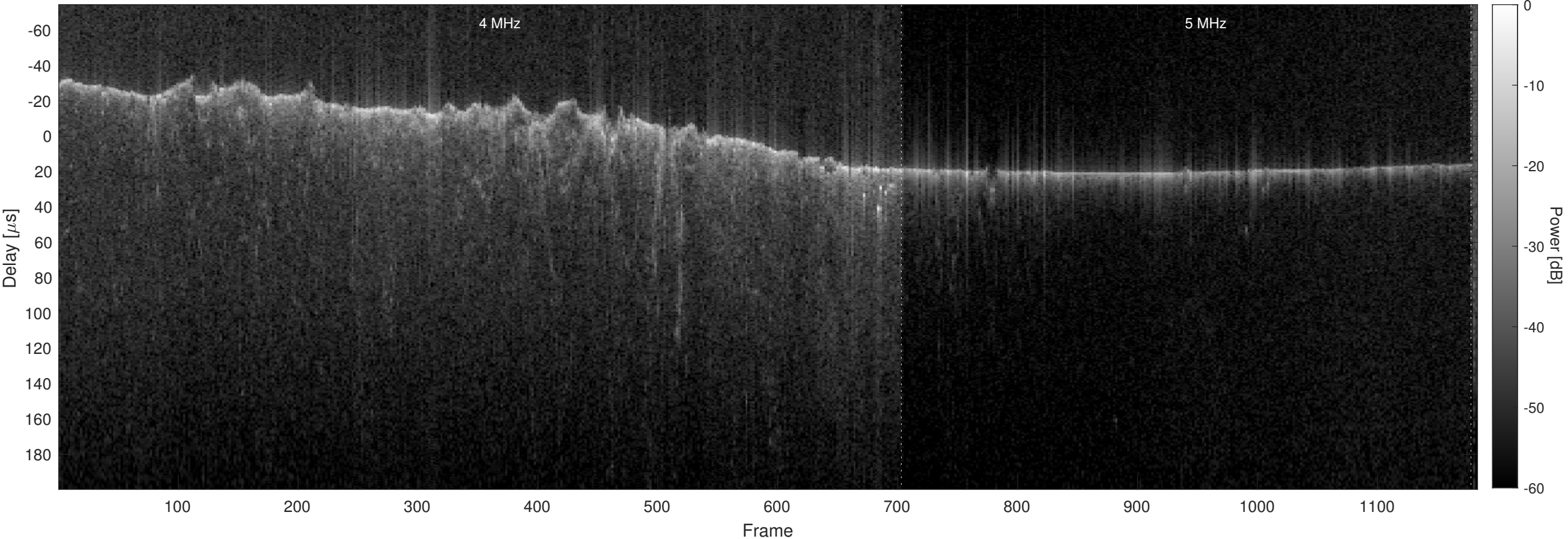
Orbit 8252, Optimized, No Window, Channel 2
