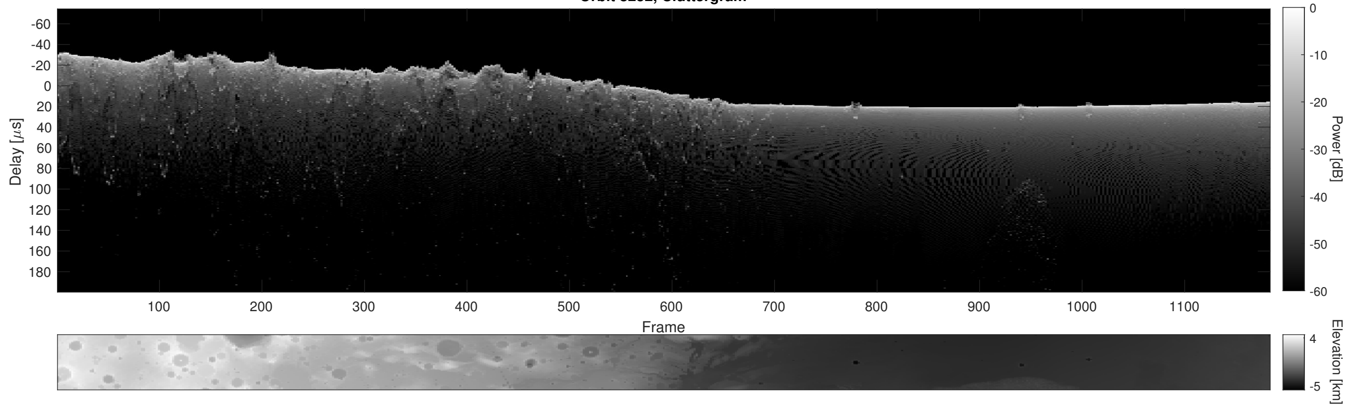
Orbit 8252, Cluttergram
