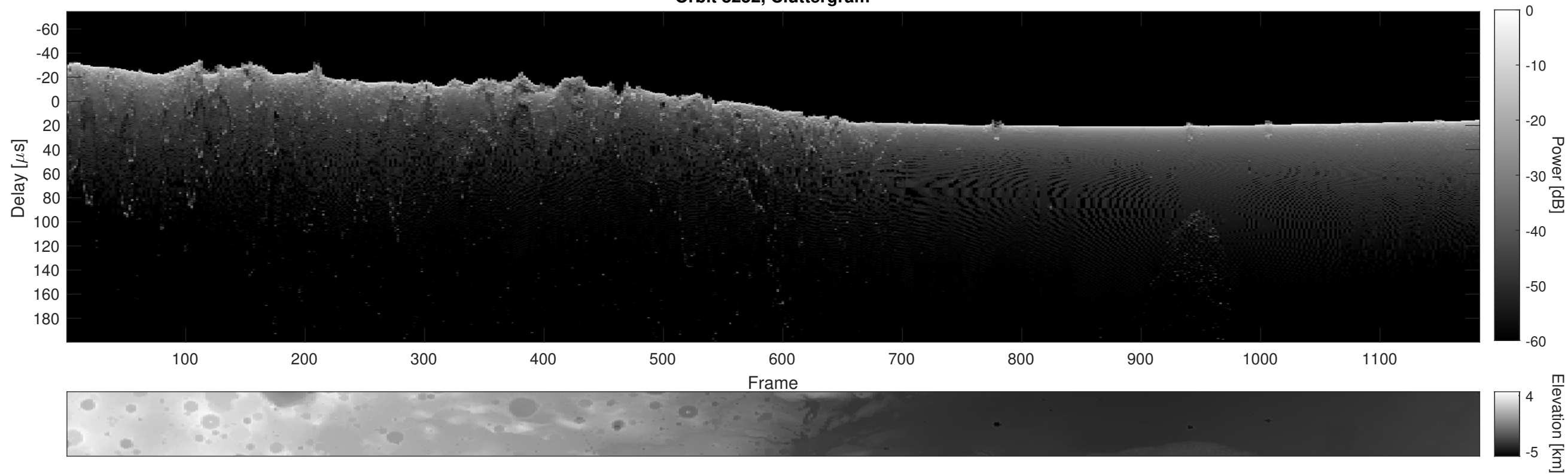
Orbit 8252, Cluttergram
