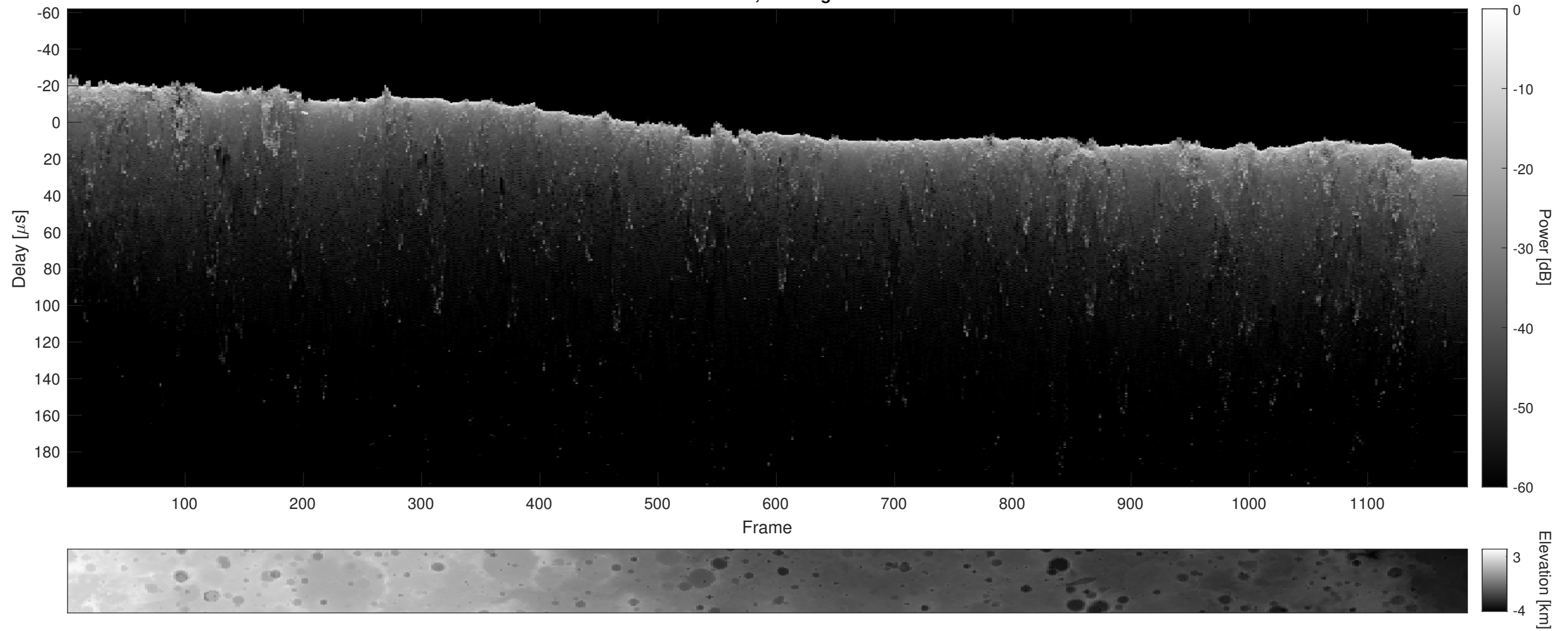
Orbit 8254, Cluttergram
