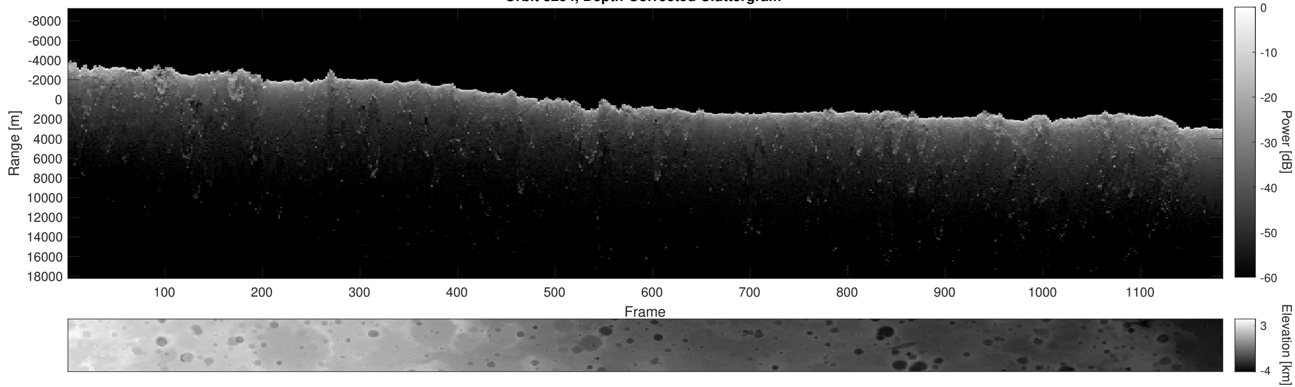
Orbit 8254, Depth-Corrected Cluttergram
