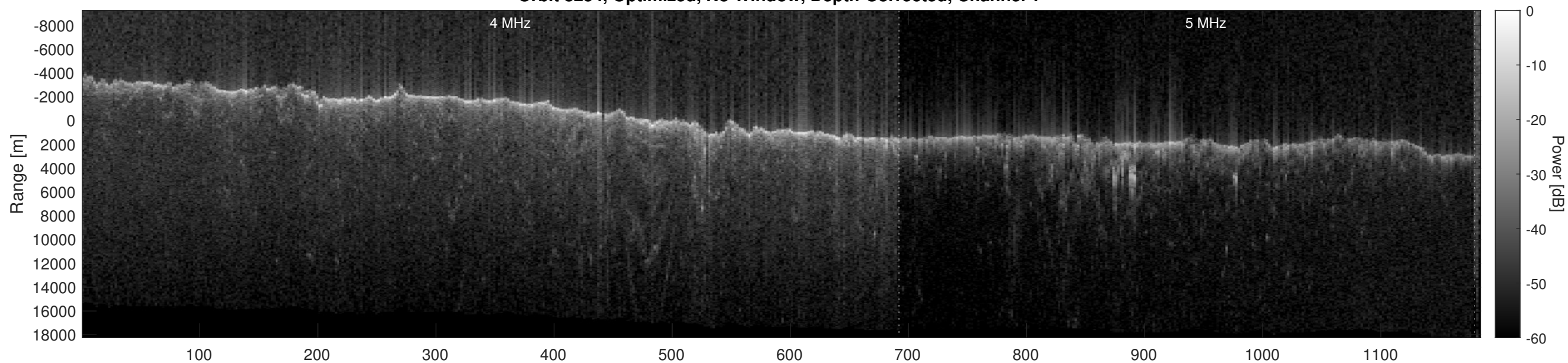
Orbit 8254, Optimized, No Window, Depth-Corrected, Channel 2
