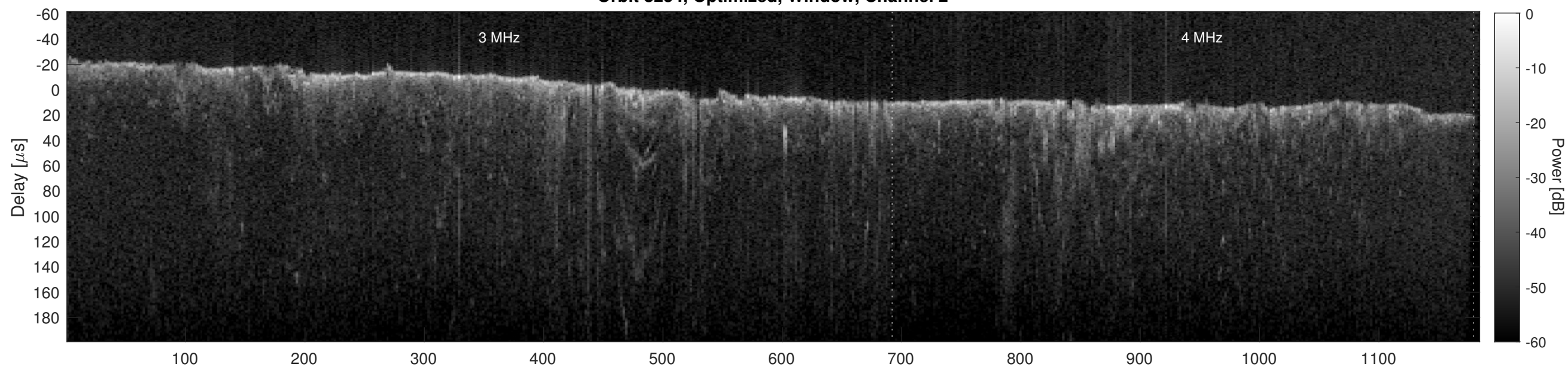
Orbit 8254, Cluttergram
