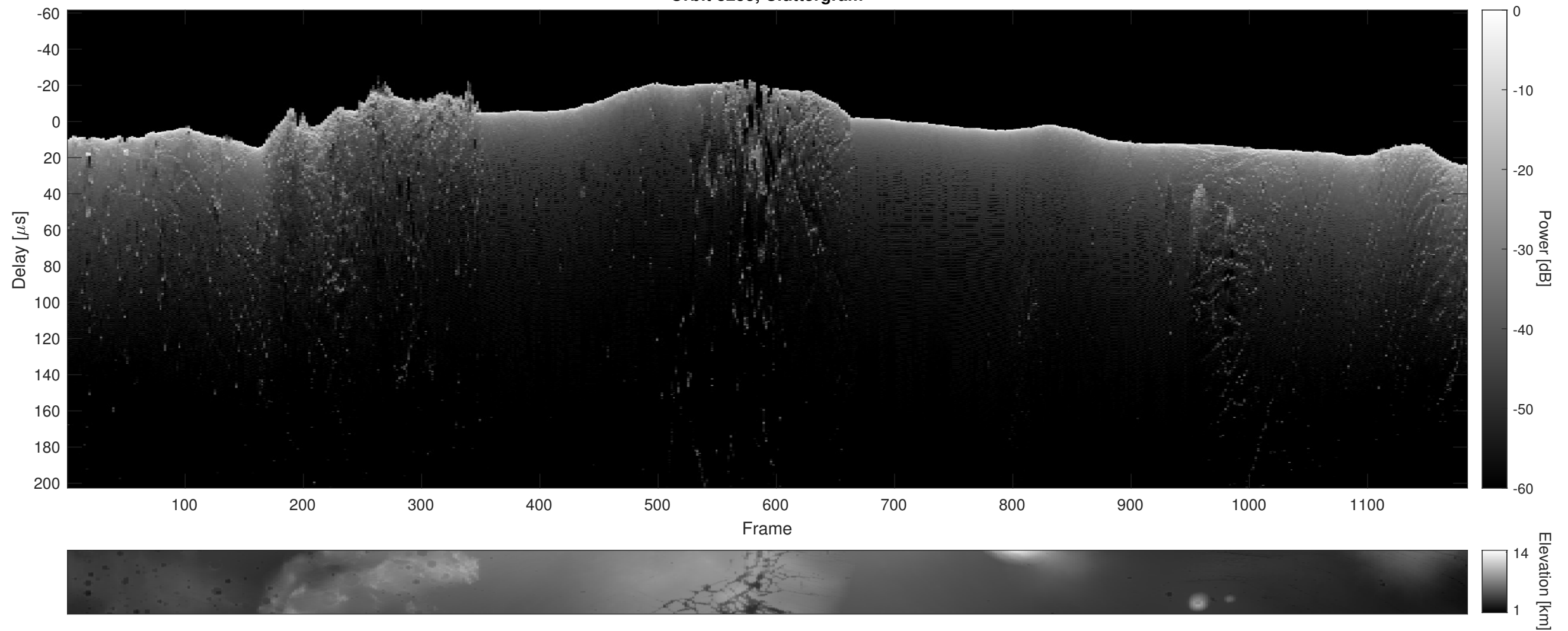
Orbit 8255, Cluttergram
