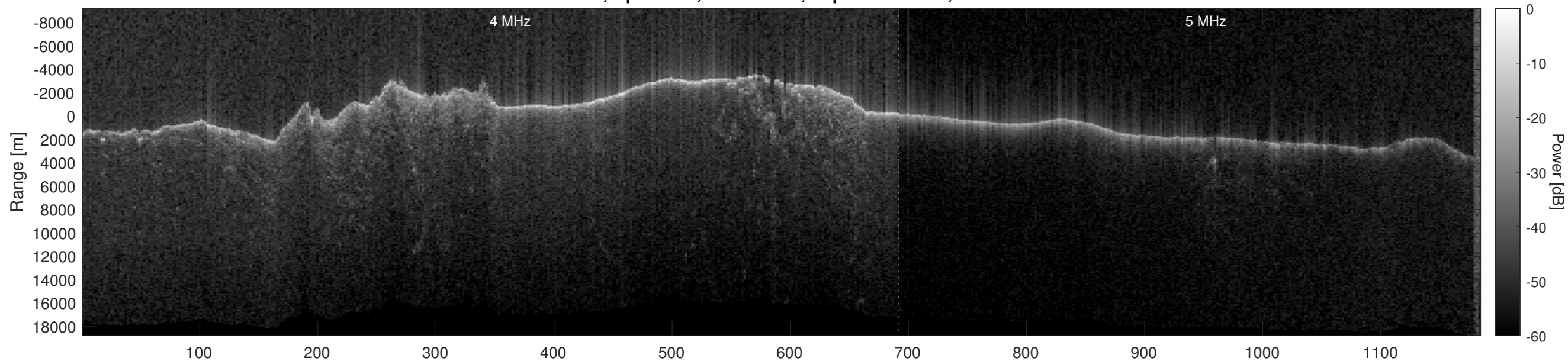
Orbit 8255, Optimized, No Window, Depth-Corrected, Channel 2
