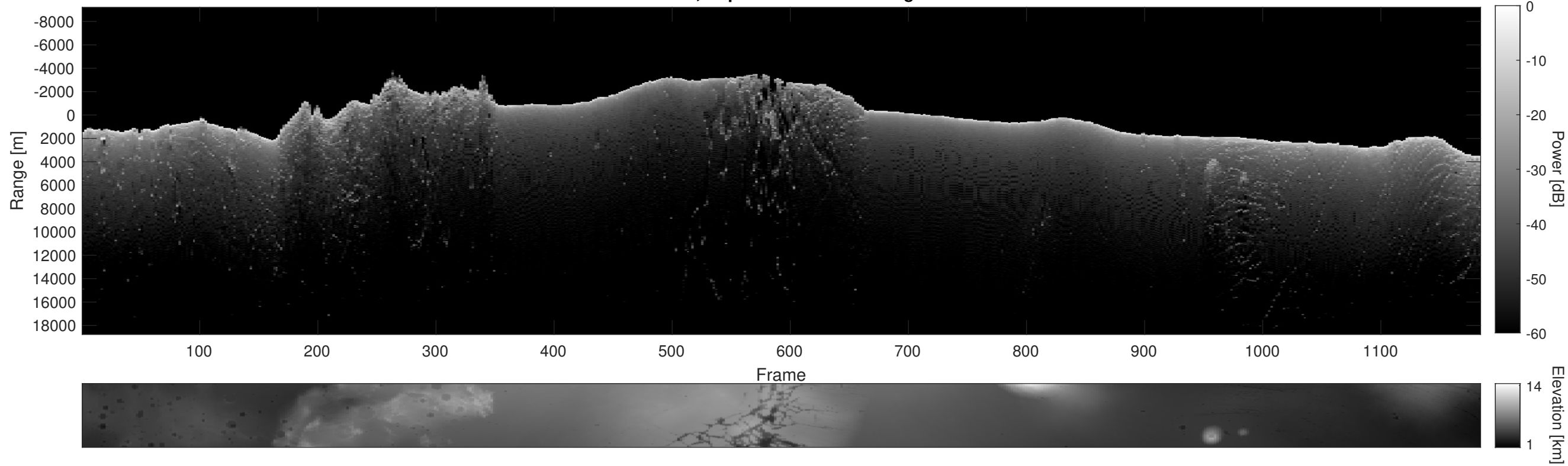
Orbit 8255, Depth-Corrected Cluttergram
