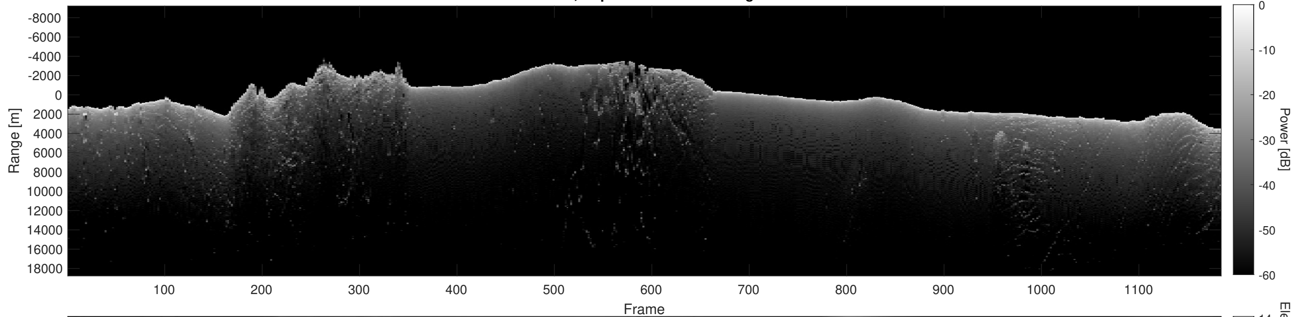
Orbit 8255, Depth-Corrected Cluttergram
