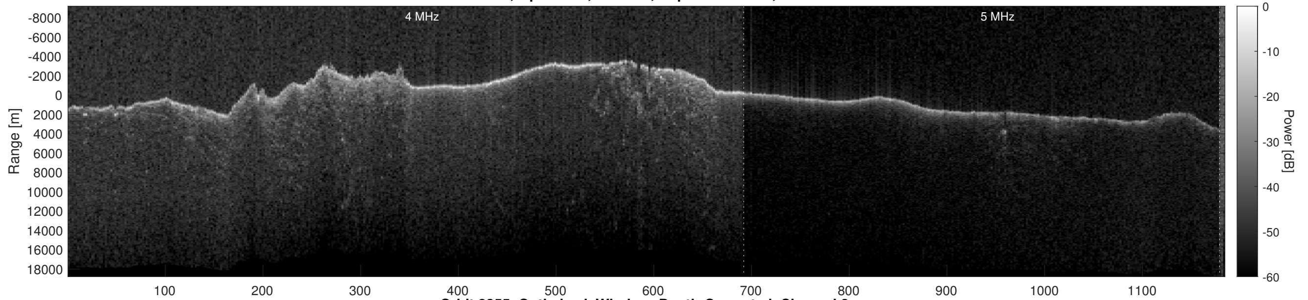
Orbit 8255, Optimized, Window, Depth-Corrected, Channel 2
