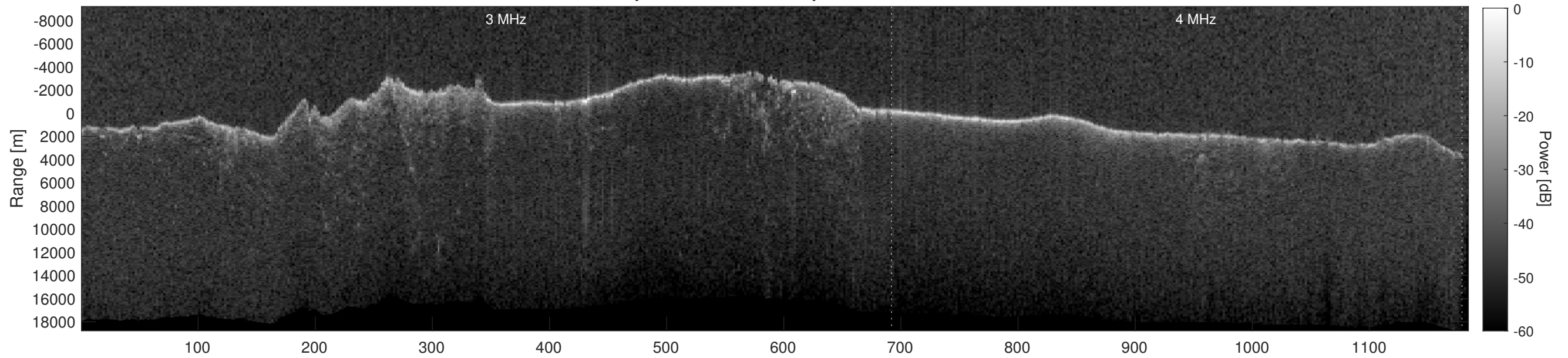
Orbit 8255, Depth-Corrected Cluttergram
