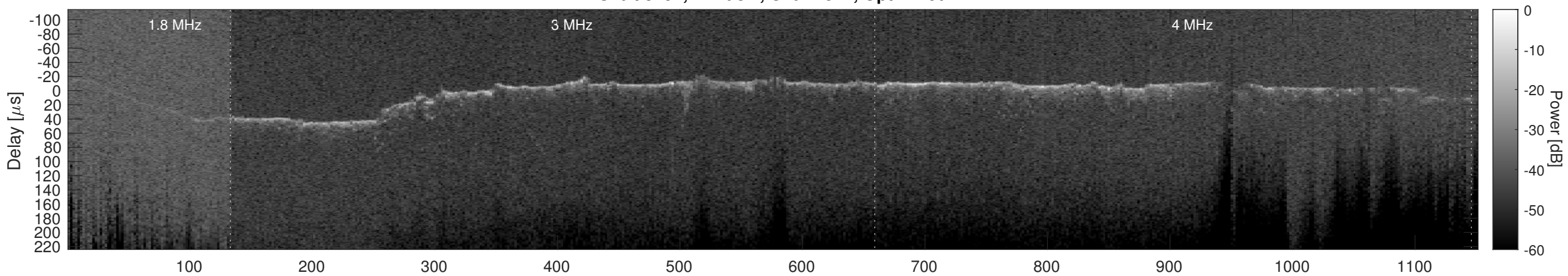
Orbit 8257, Cluttergram
