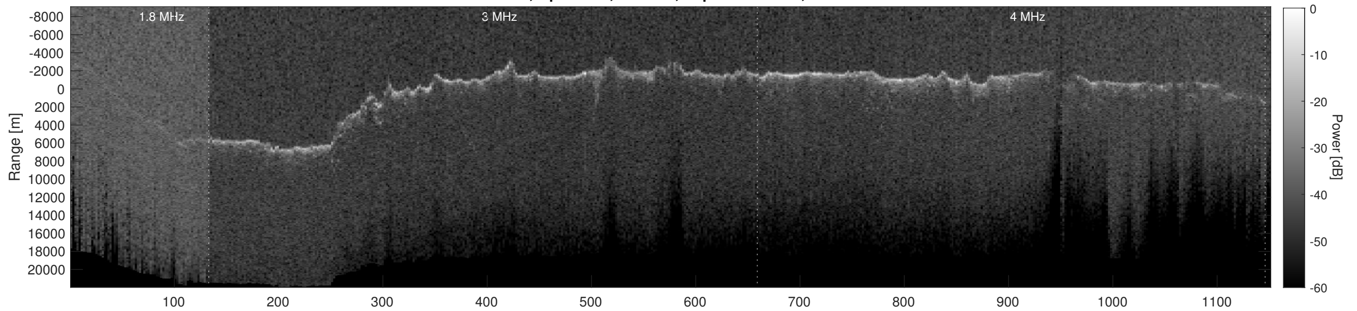
Orbit 8257, Depth-Corrected Cluttergram
