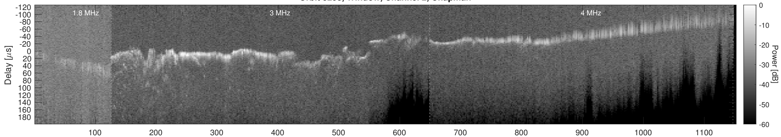
Orbit 8258, Window, Channel 2, Optimized
