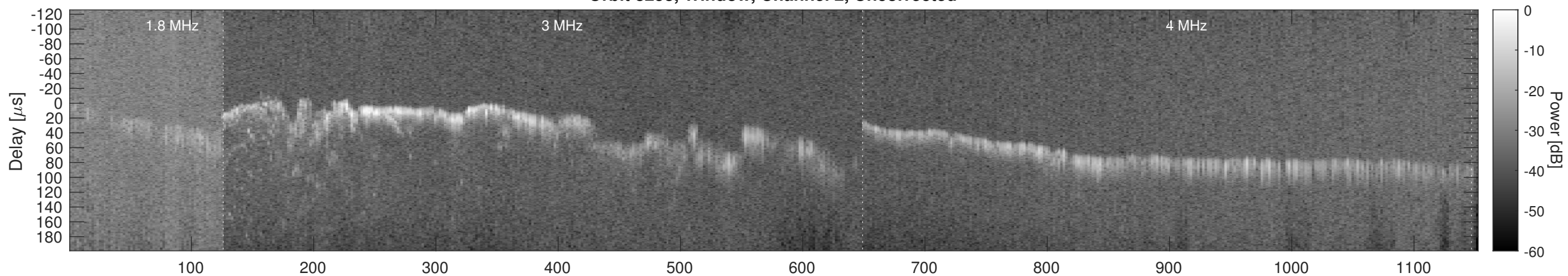
Orbit 8258, Window, Channel 2, Chapman
