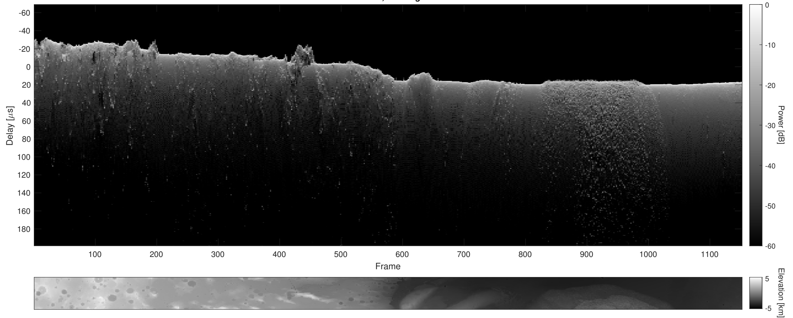
Orbit 8259, Cluttergram
