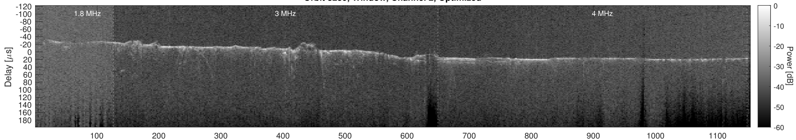
Orbit 8259, Cluttergram
