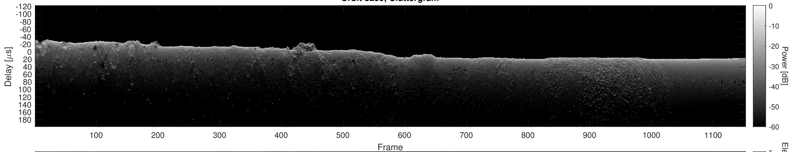
Orbit 8259, Cluttergram
