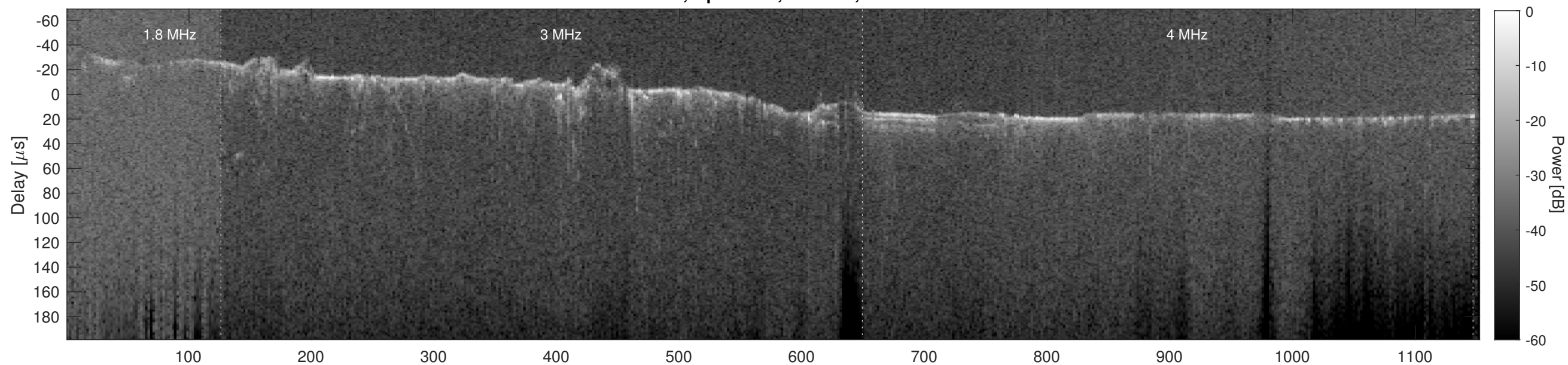
Orbit 8259, Cluttergram
