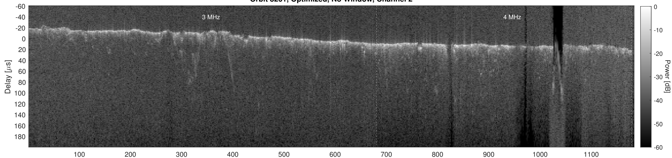
Orbit 8261, Cluttergram
