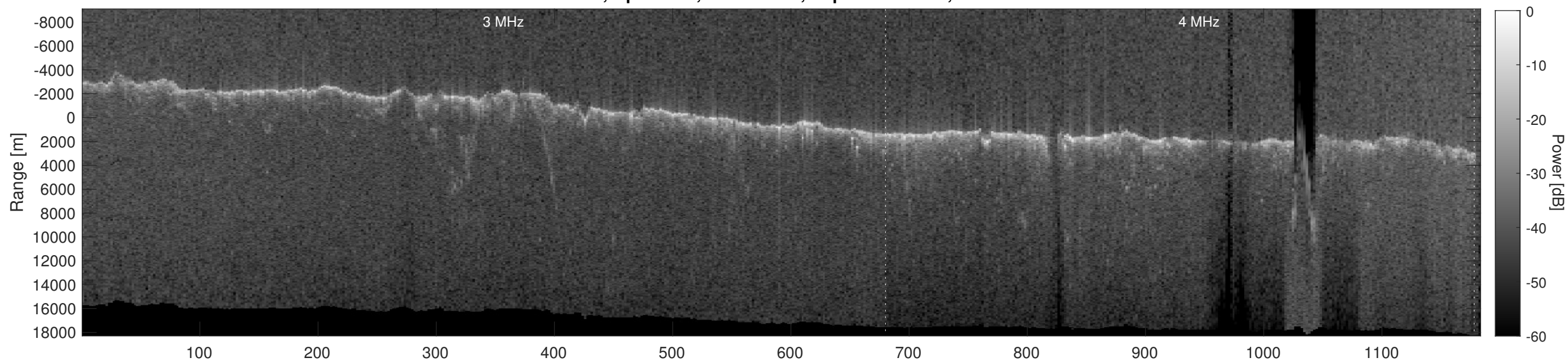
Orbit 8261, Depth-Corrected Cluttergram
