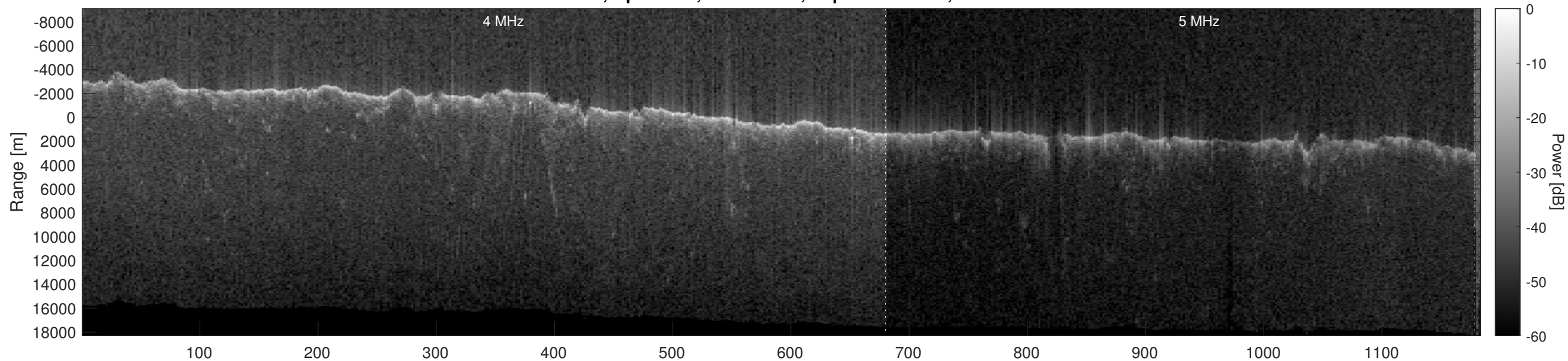
Orbit 8261, Optimized, No Window, Depth-Corrected, Channel 2
