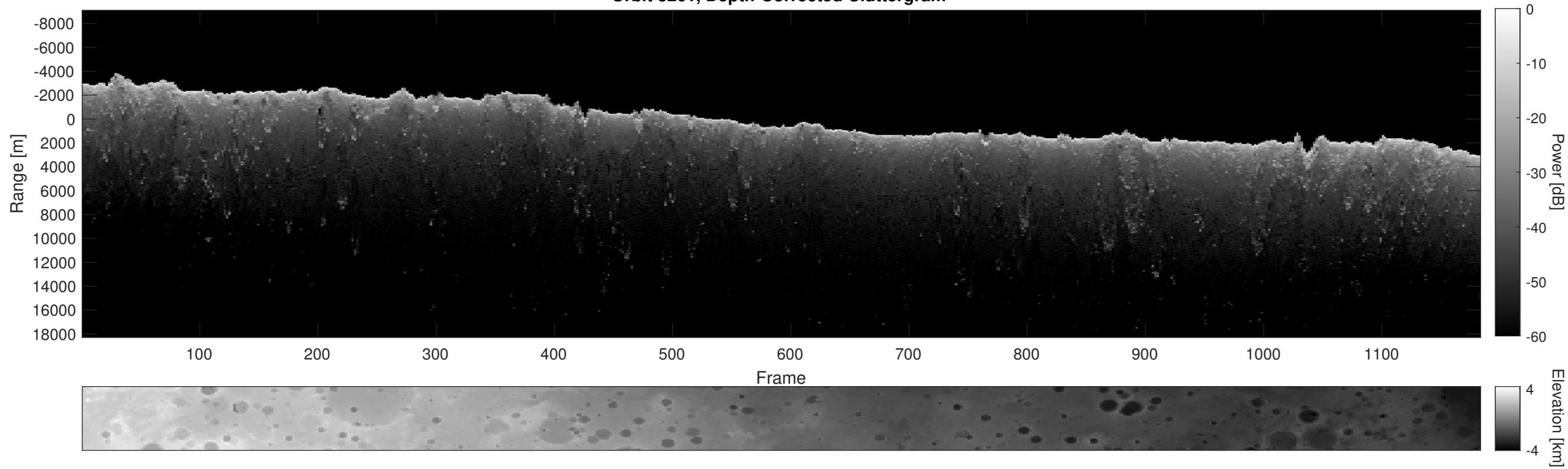
Orbit 8261, Depth-Corrected Cluttergram
