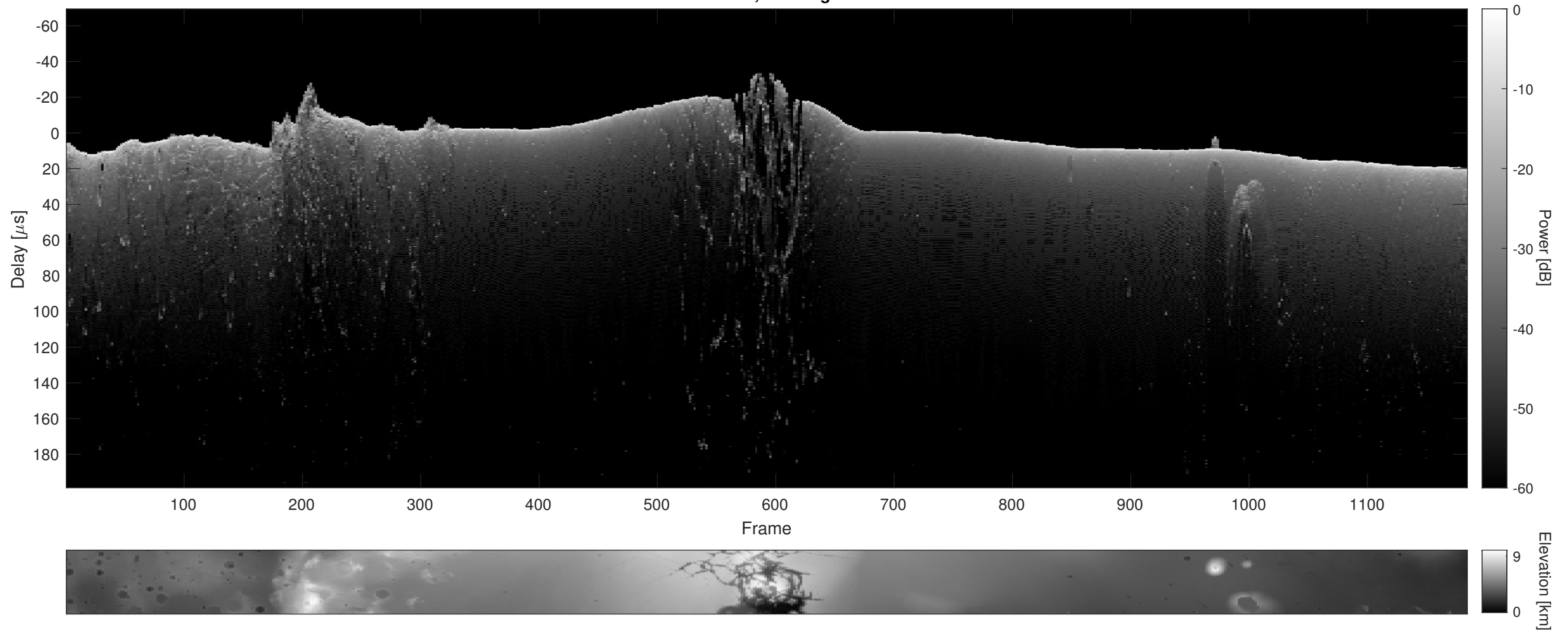
Orbit 8262, Cluttergram
