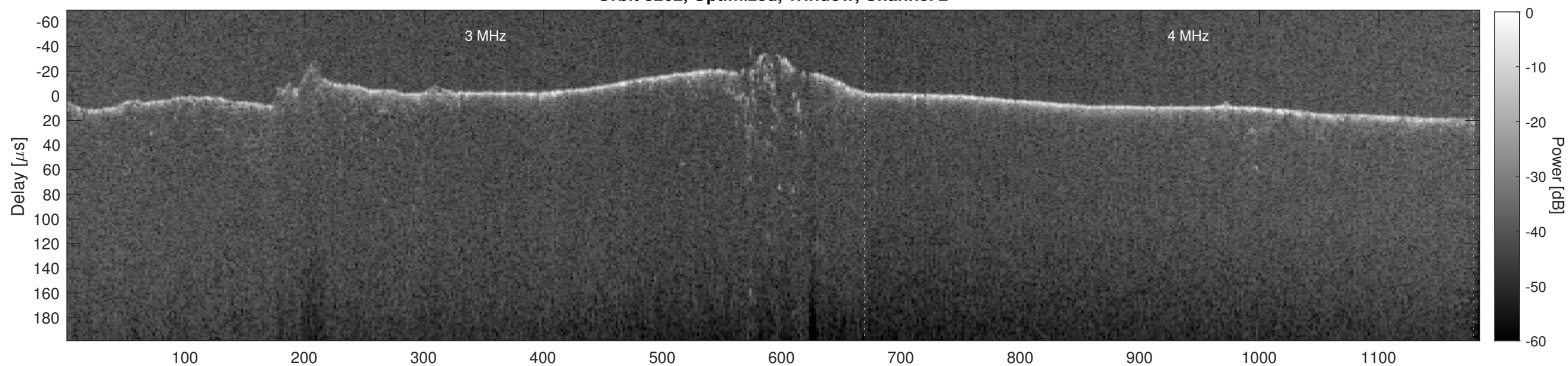
Orbit 8262, Cluttergram
