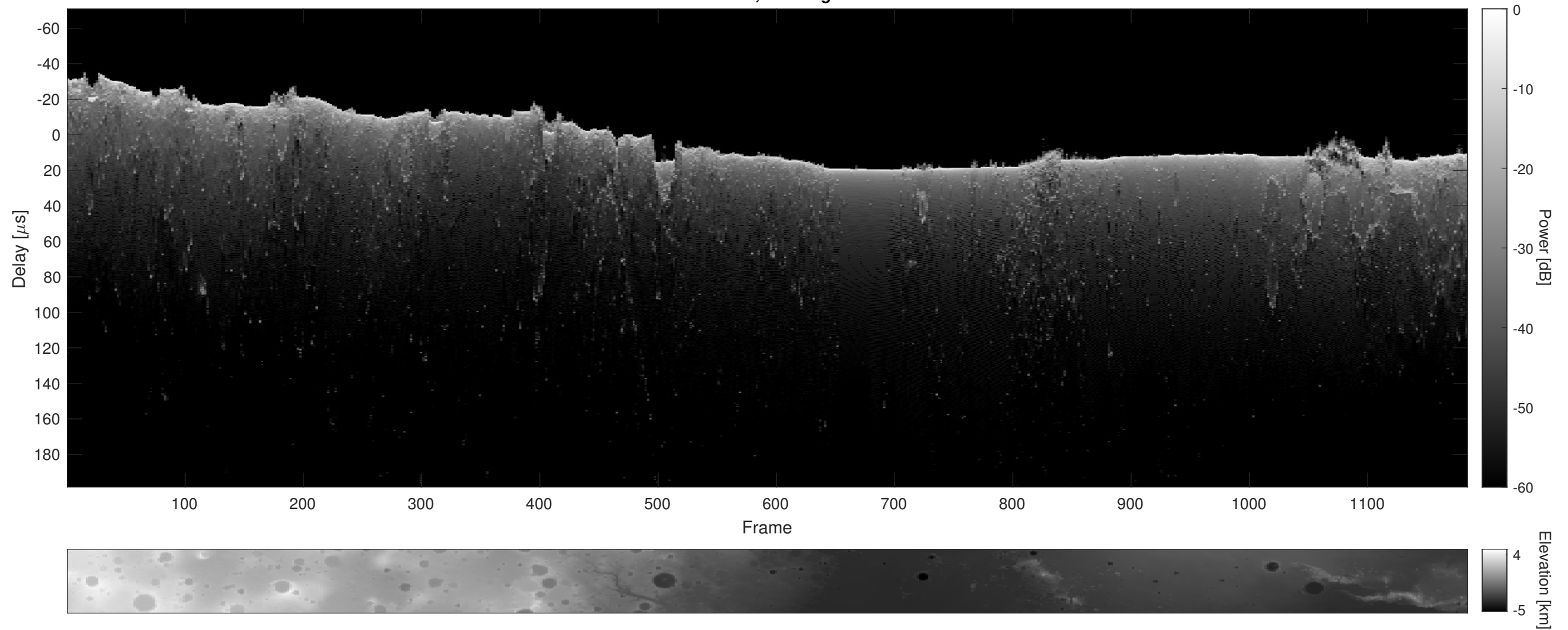
Orbit 8263, Cluttergram
