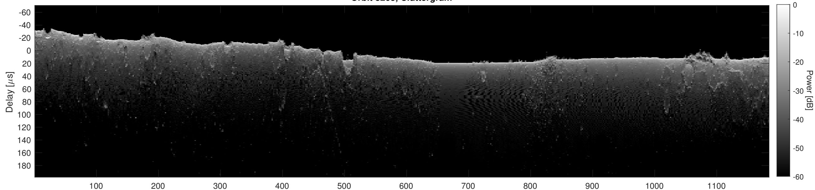
Orbit 8263, Cluttergram
