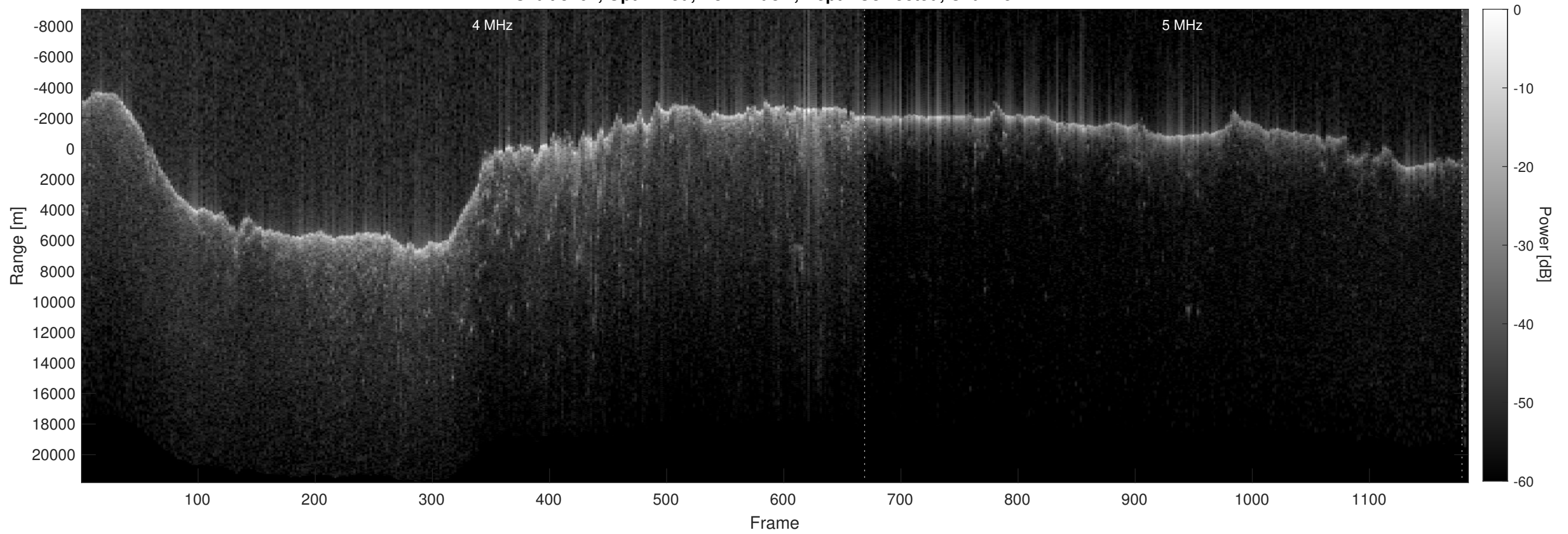
Orbit 8264, Optimized, No Window, Depth-Corrected, Channel 2
