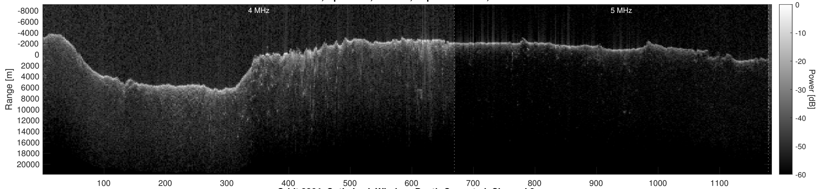
Orbit 8264, Optimized, Window, Depth-Corrected, Channel 2
