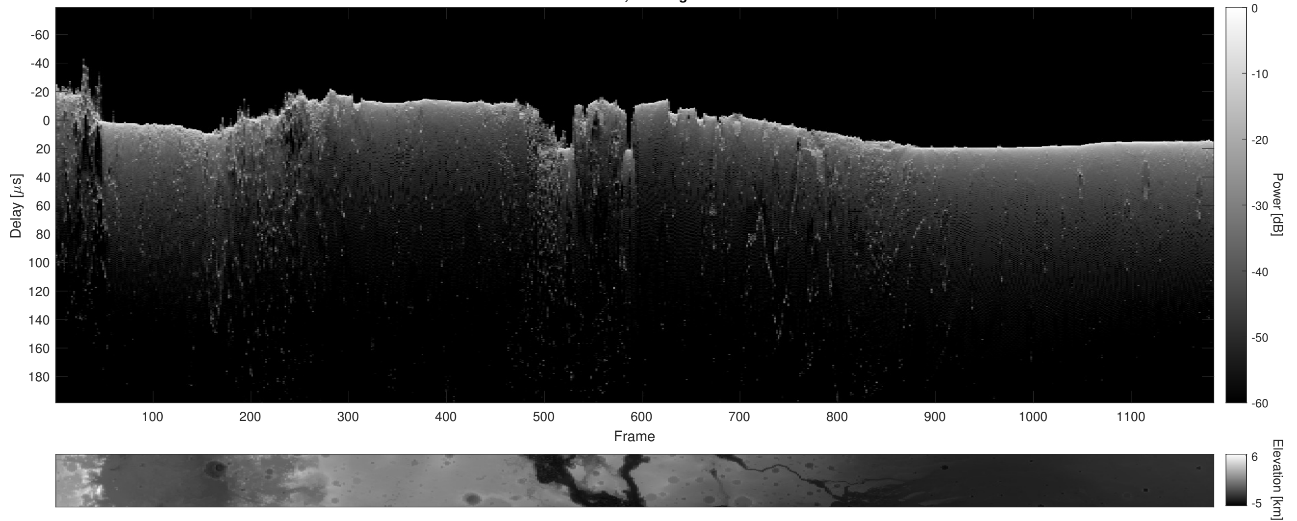
Orbit 8265, Cluttergram
