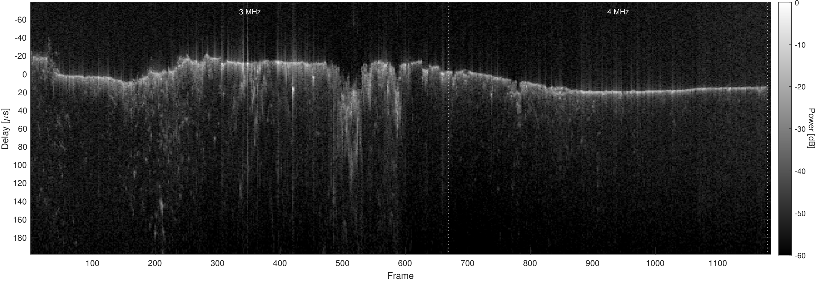
Orbit 8265, Optimized, No Window, Channel 2
