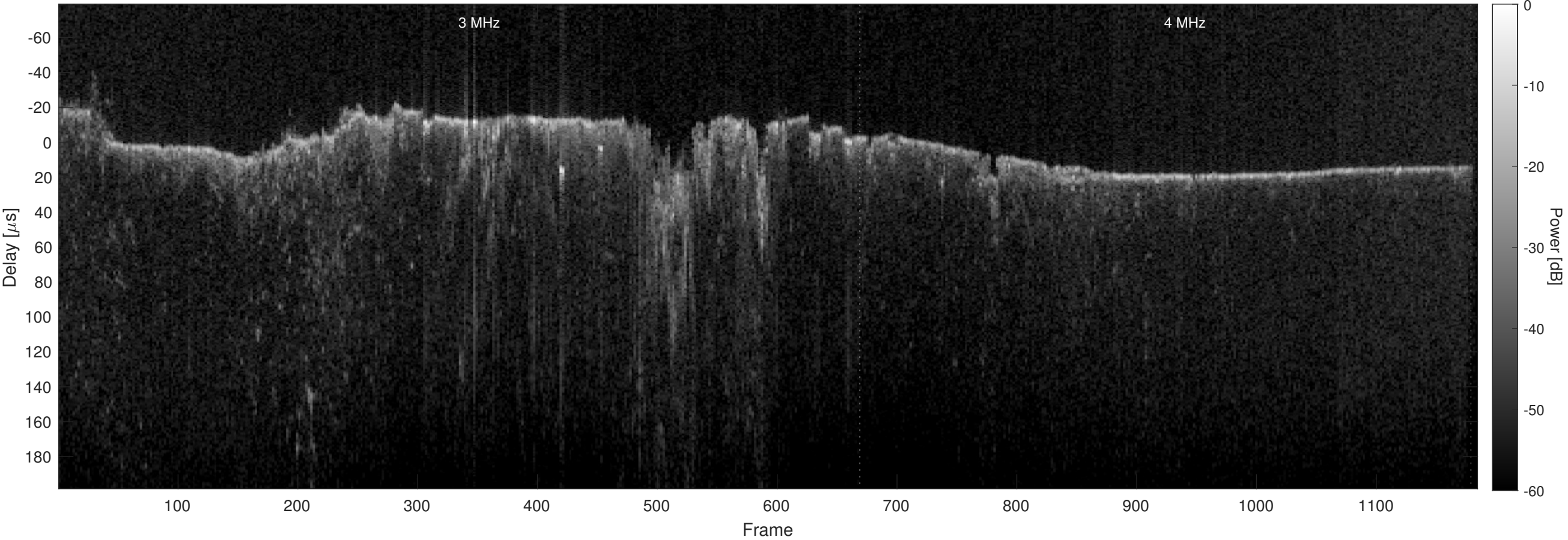
Orbit 8265, Optimized, Window, Channel 2
