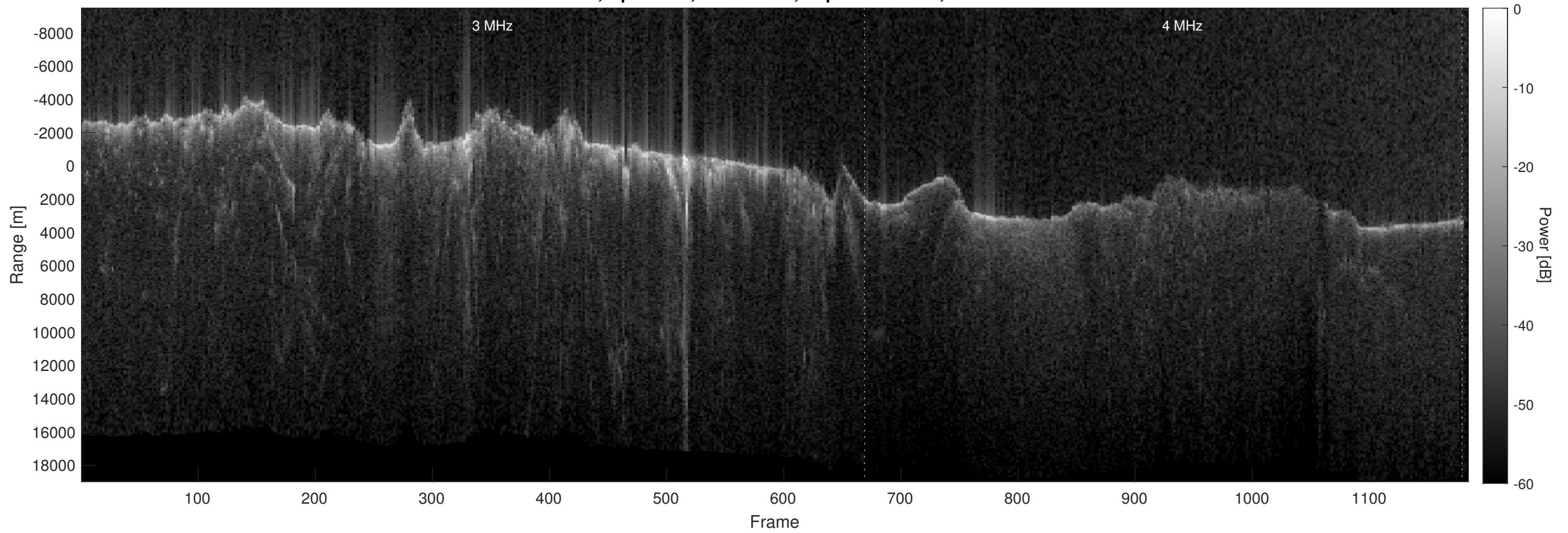
Orbit 8266, Optimized, No Window, Depth-Corrected, Channel 2
