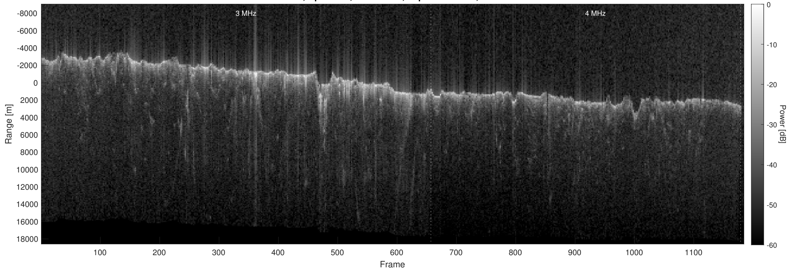
Orbit 8268, Optimized, No Window, Depth-Corrected, Channel 2
