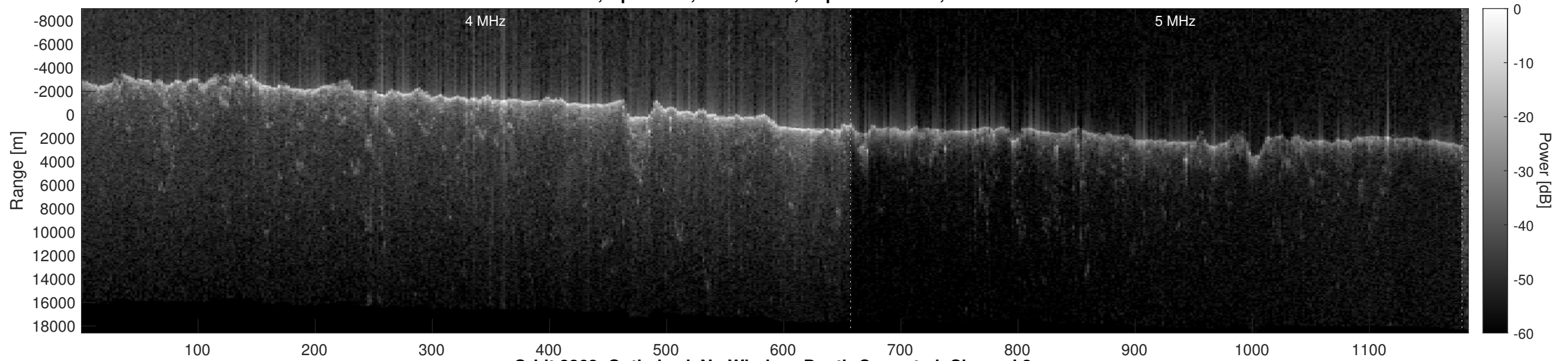
Orbit 8268, Optimized, No Window, Depth-Corrected, Channel 2
