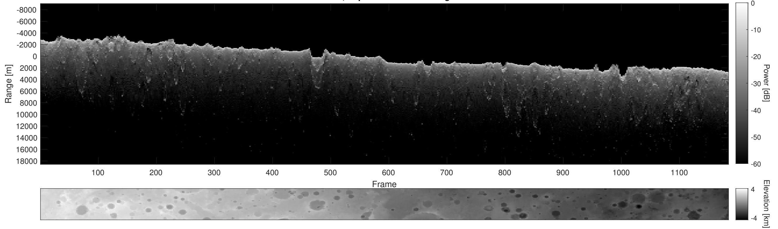
Orbit 8268, Depth-Corrected Cluttergram
