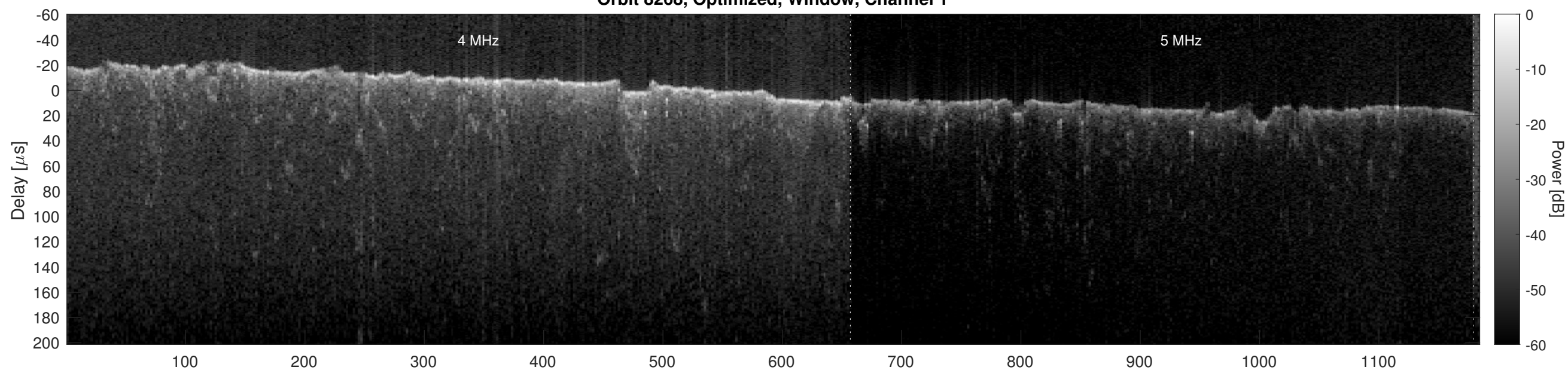
Orbit 8268, Optimized, Window, Channel 2
