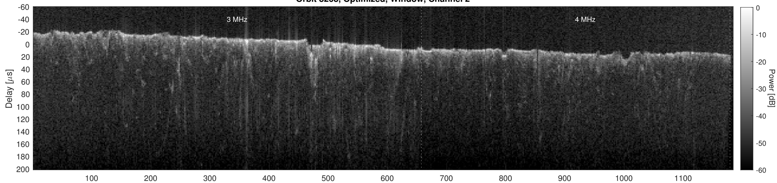
Orbit 8268, Cluttergram
