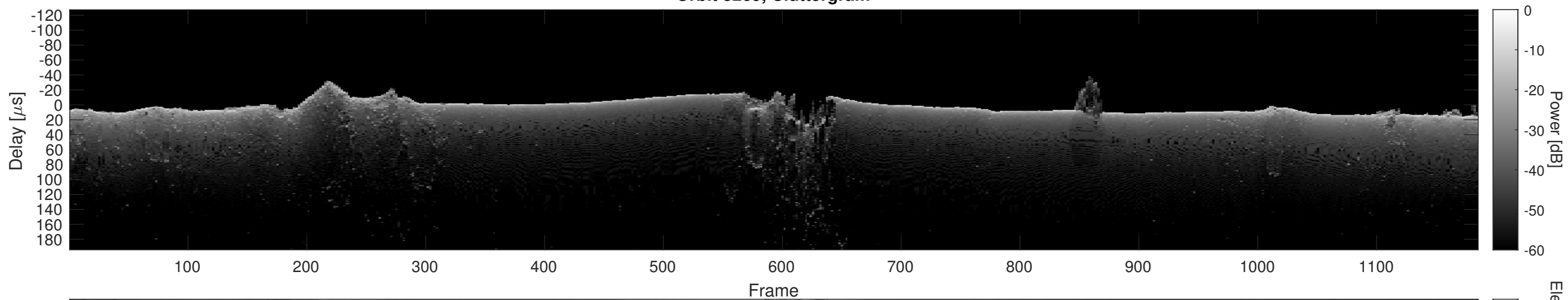
Orbit 8269, Cluttergram
