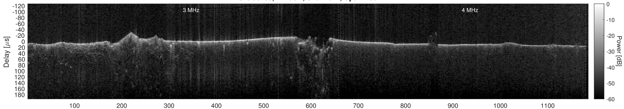
Orbit 8269, Cluttergram
