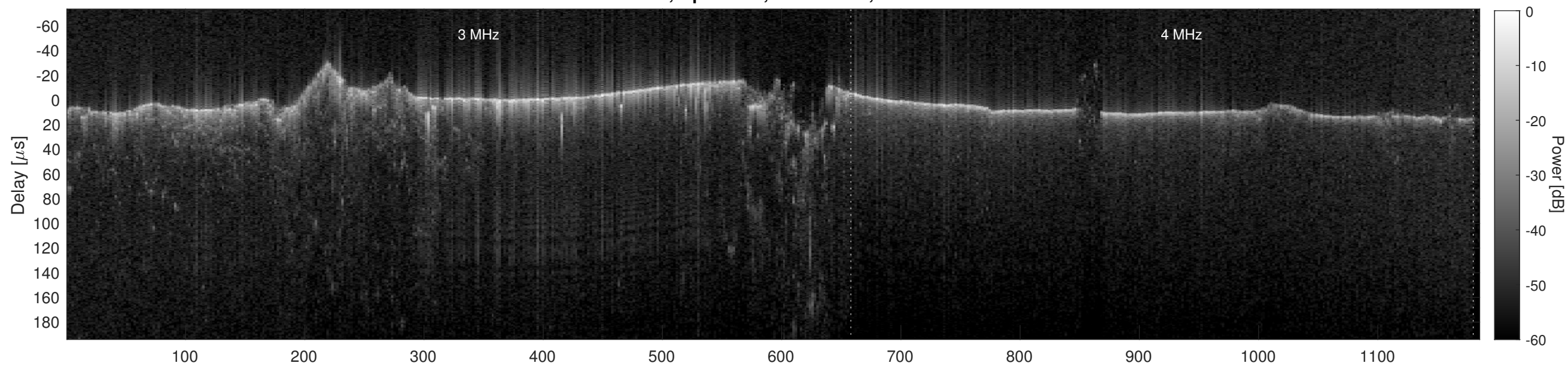
Orbit 8269, Cluttergram
