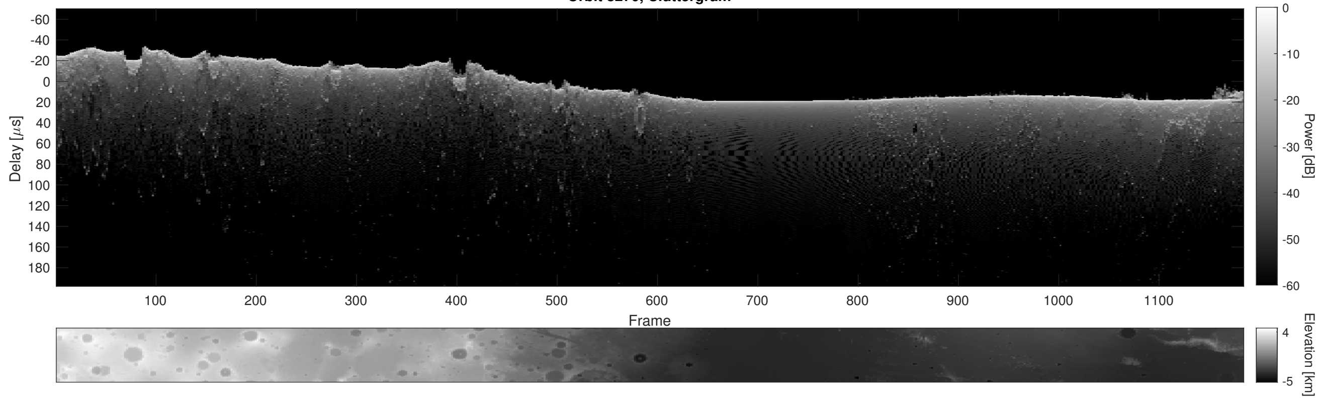
Orbit 8270, Cluttergram
