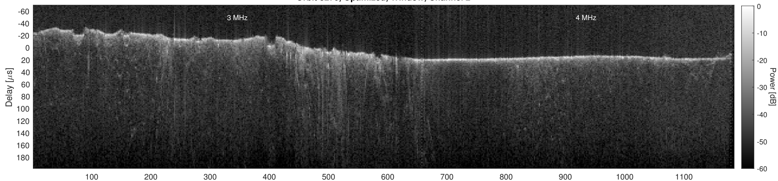
Orbit 8270, Cluttergram
