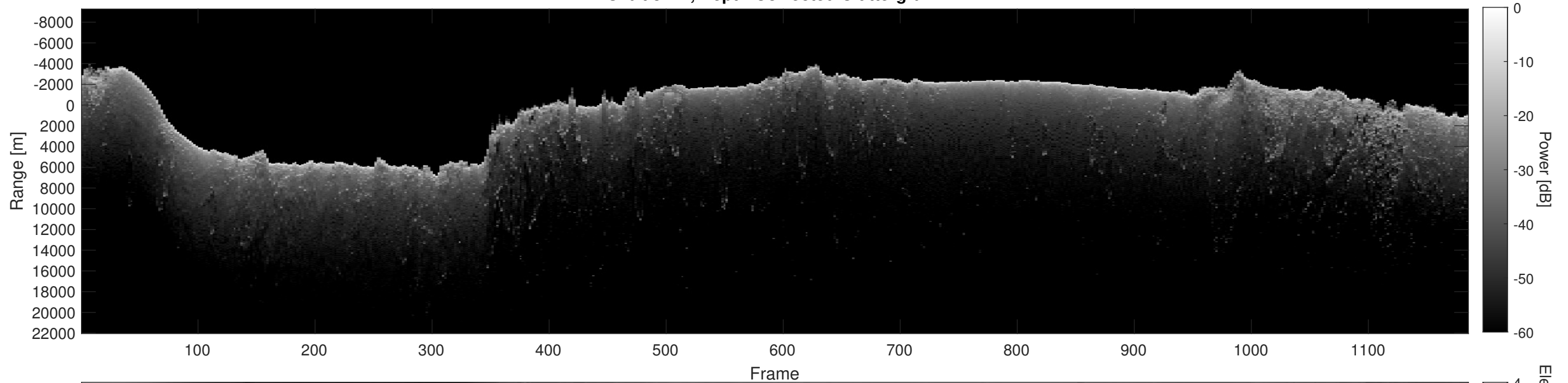
Orbit 8271, Depth-Corrected Cluttergram
