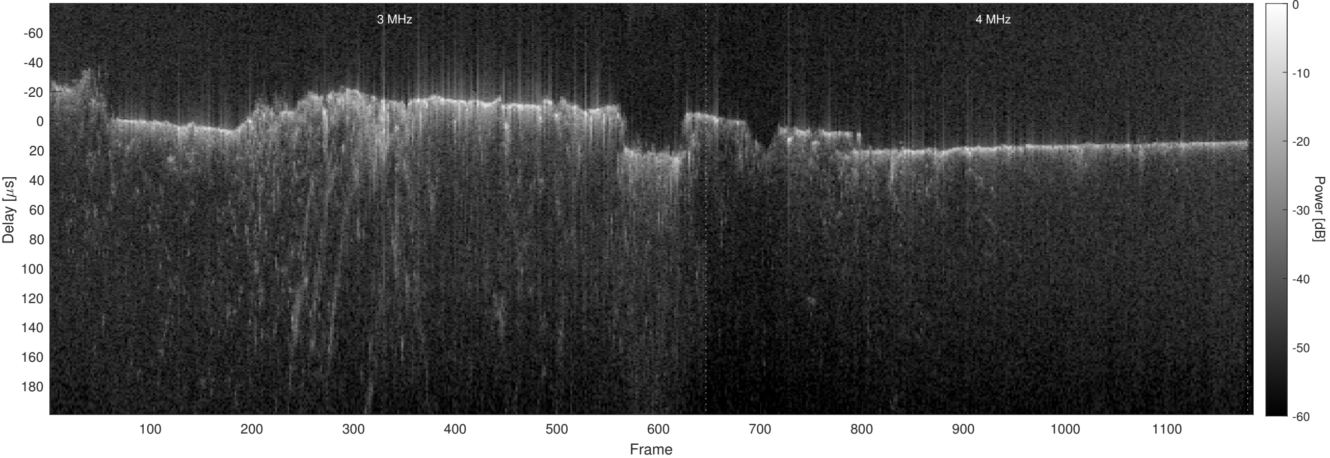
Orbit 8272, Optimized, No Window, Channel 2
