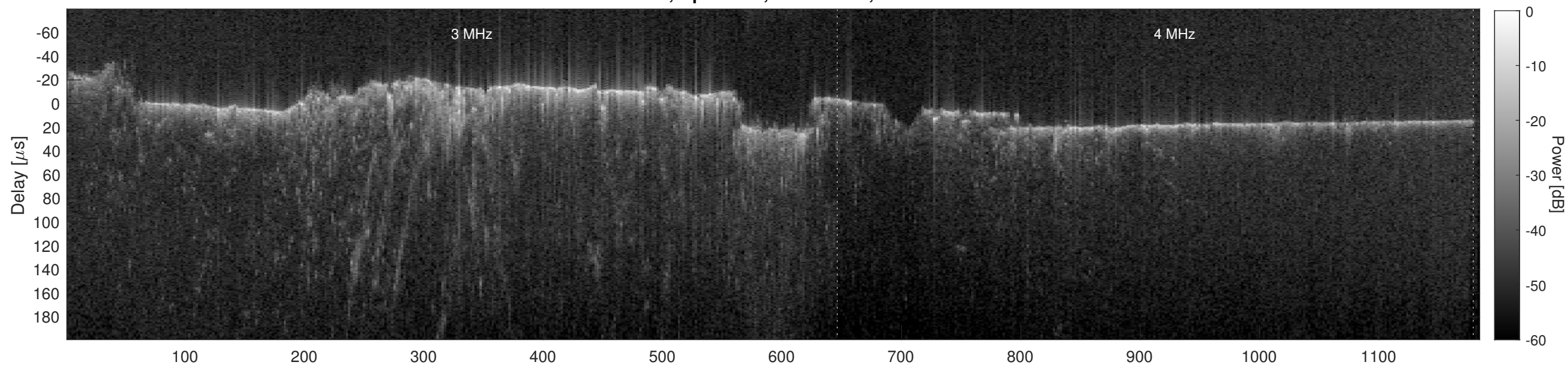
Orbit 8272, Cluttergram
