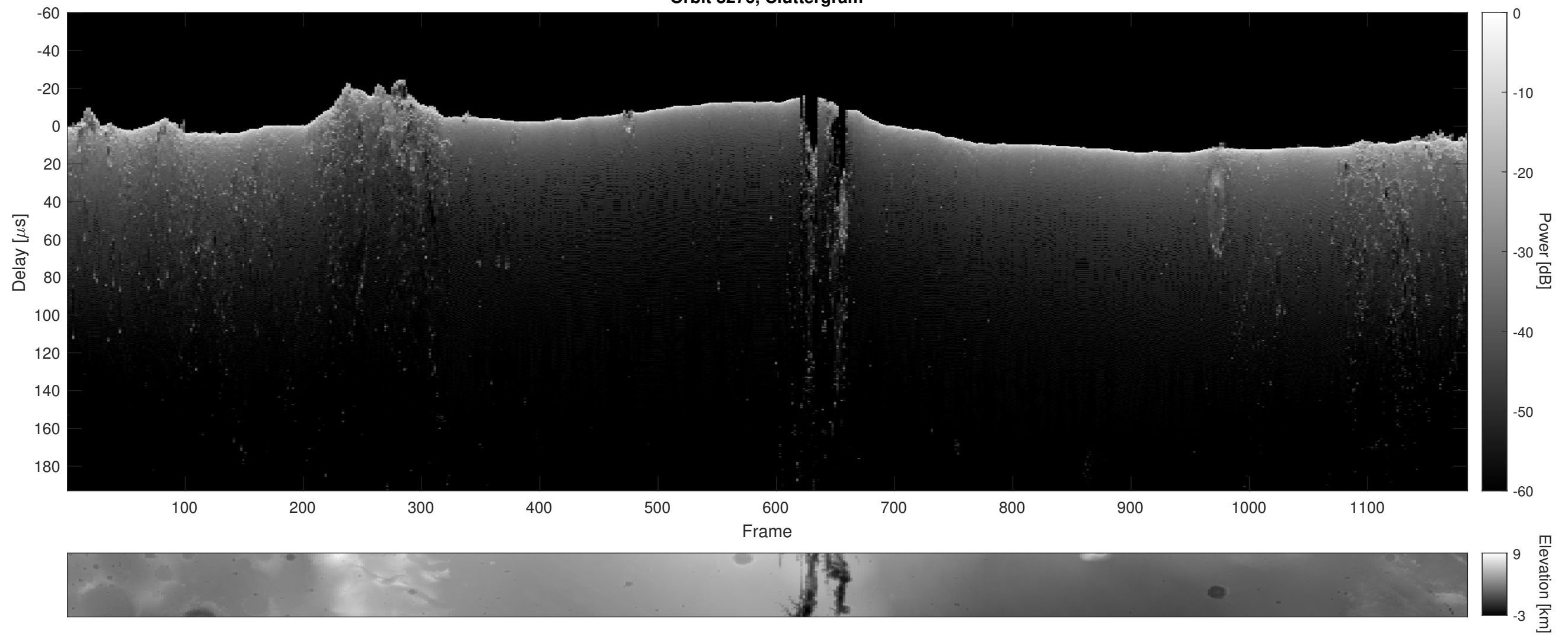
Orbit 8276, Cluttergram
