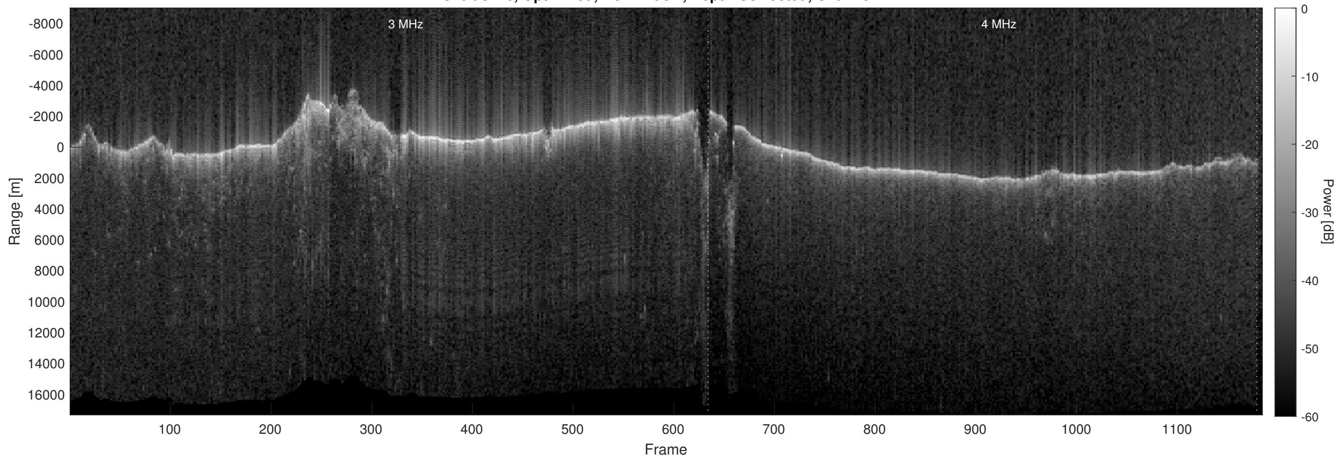
Orbit 8276, Optimized, No Window, Depth-Corrected, Channel 2
