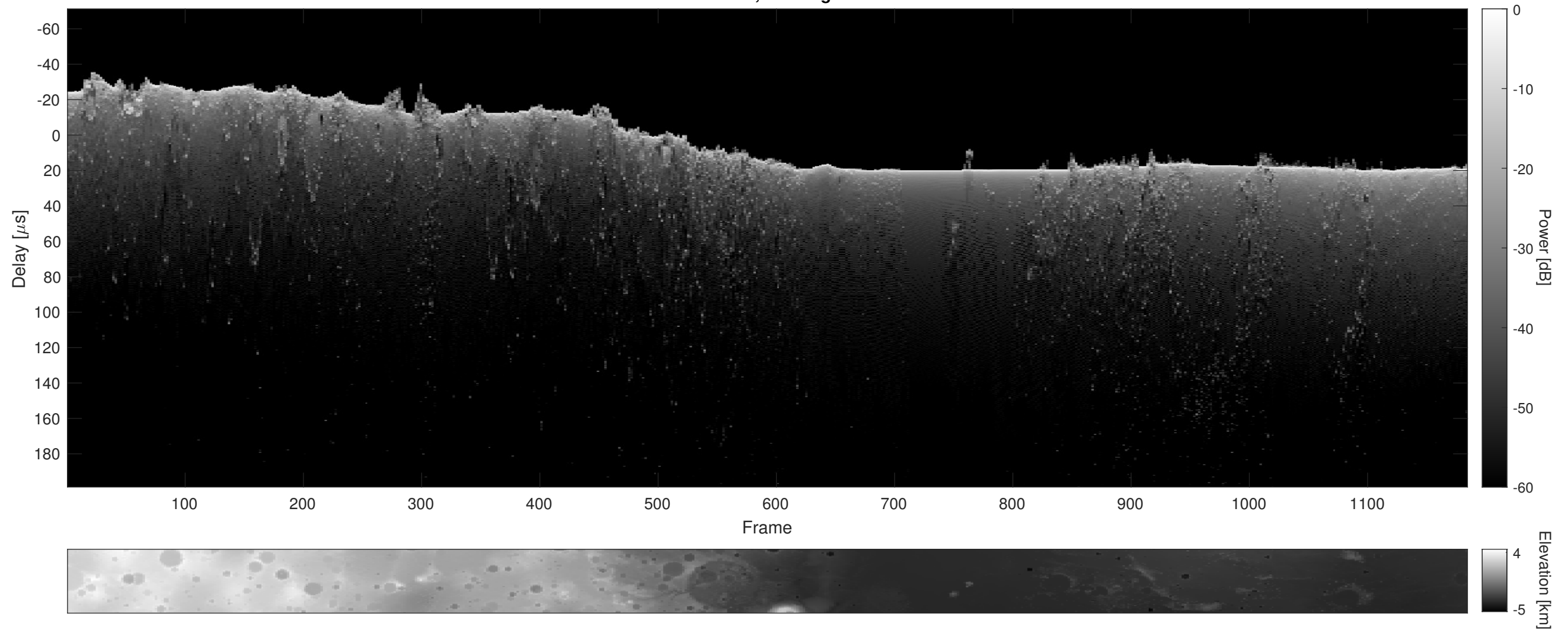
Orbit 8277, Cluttergram
