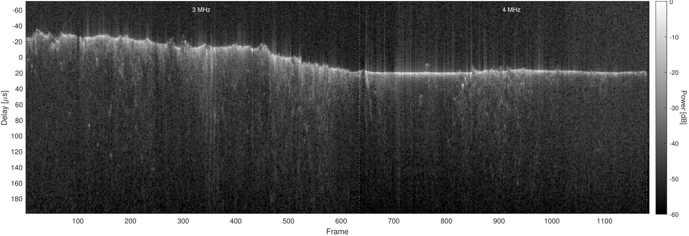
Orbit 8277, Optimized, No Window, Channel 2
