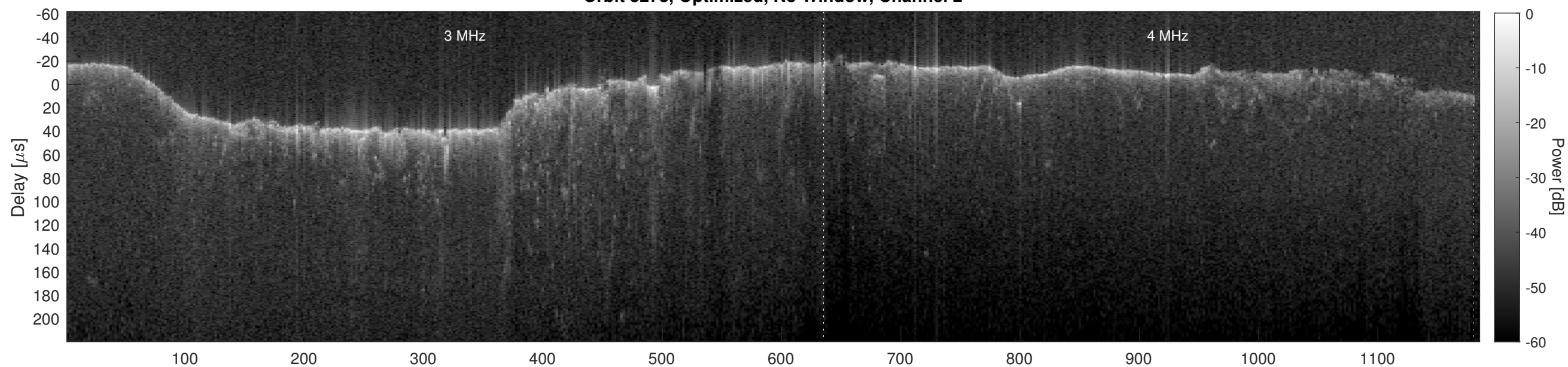
Orbit 8278, Cluttergram
